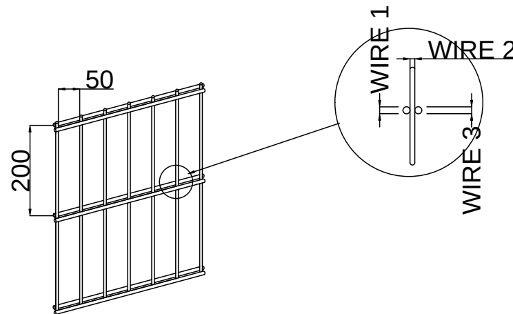
MESH DETAILS
