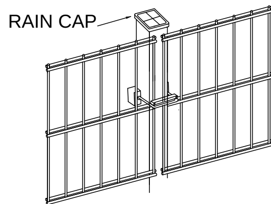
ASSEMBLY DETAIL 2
