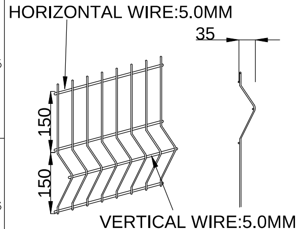
DETAIL 01
