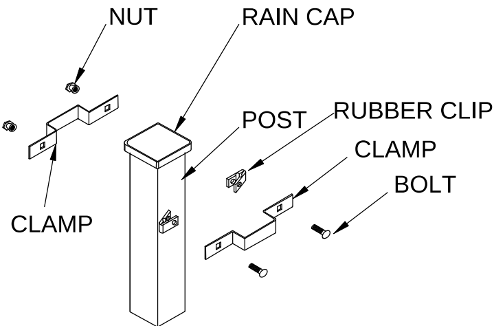
DETAIL 02
