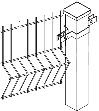
DETAIL 02
